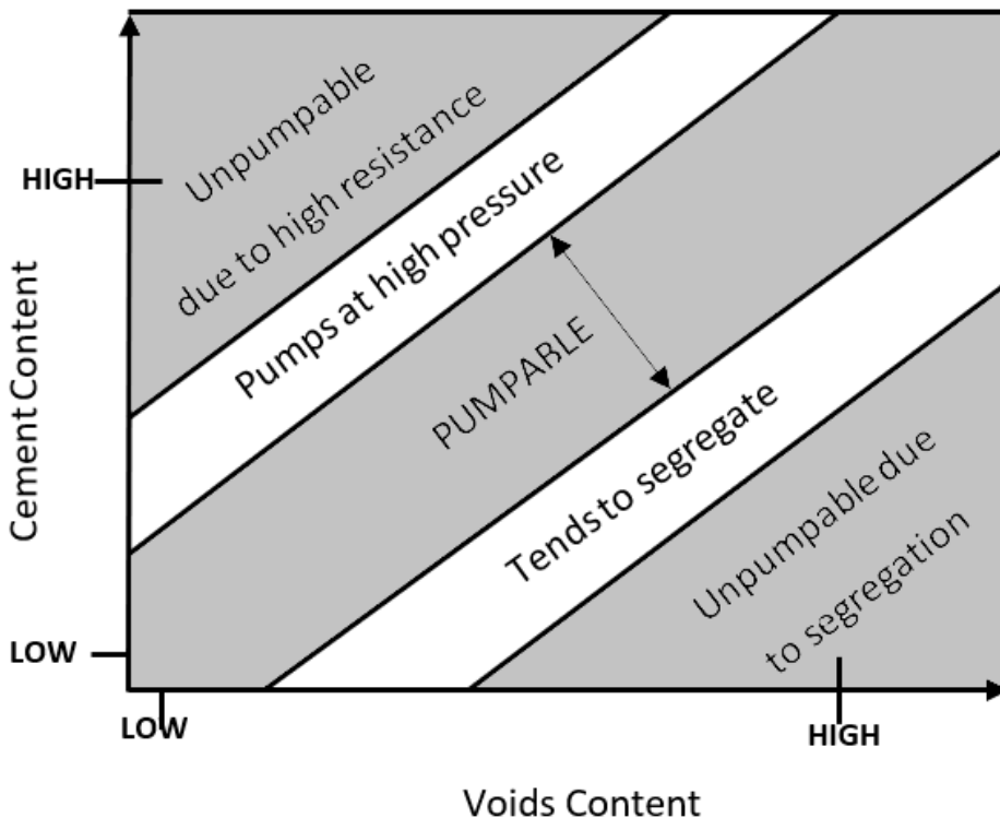
Diagrammatic illustration of the behaviour of given materials when pumped.
